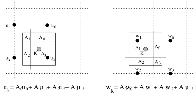
Figure 3: Area weighting interpolation scheme for determining local fluid velocity for a marker k .
